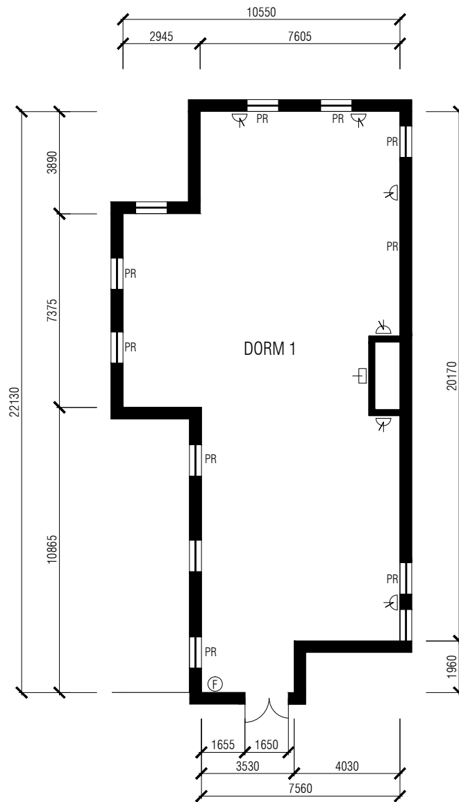
ROSINA DORM 1 PLAN
