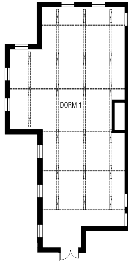
ROSINA DORM 1 REFLECTED CEILING PLAN
