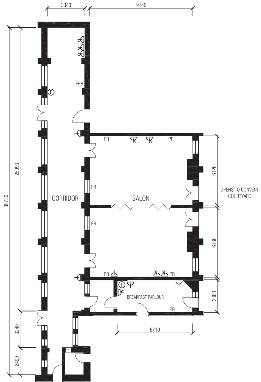
CONVENT SALON, CORRIDOR, AND BREAKFAST PARLOUR PLAN
