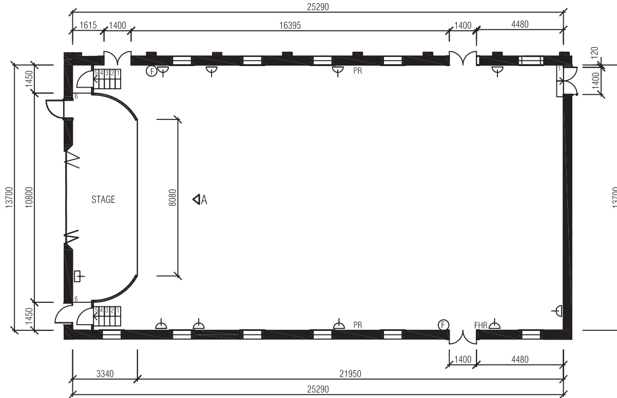
ROSINA AUDITORIUM PLAN
