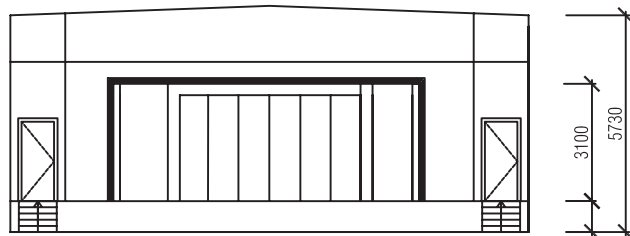
PERFORMANCE HALL WEST INTERIOR ELEVATION A
